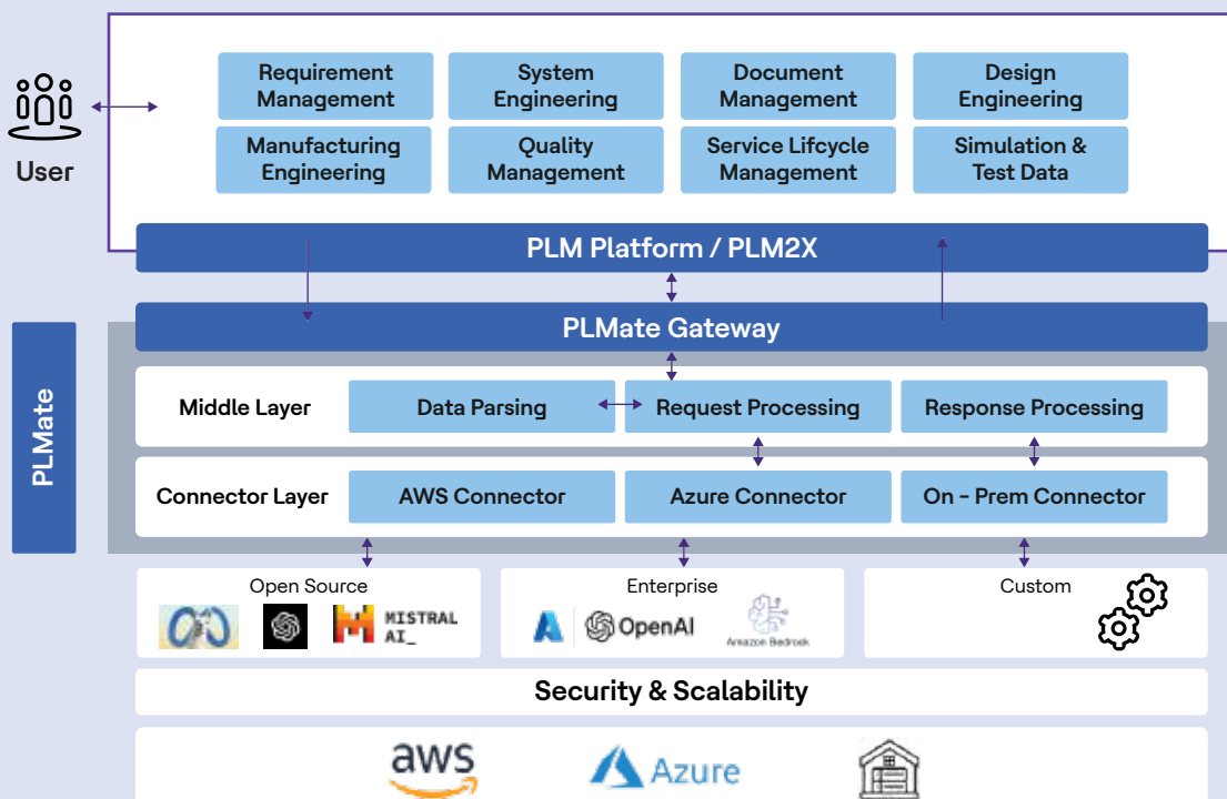
HCLTech PLMate solution architecture diagram
