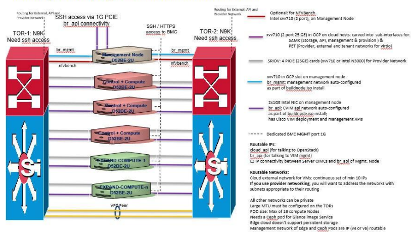
Quanta (D52BE-2U) edge Pod with 25GE Intel NIC and N3000
