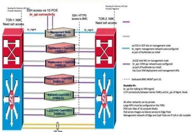
Quanta (D52BQ-2U) ceph Pod with 25GE Intel NIC (xxv710)
