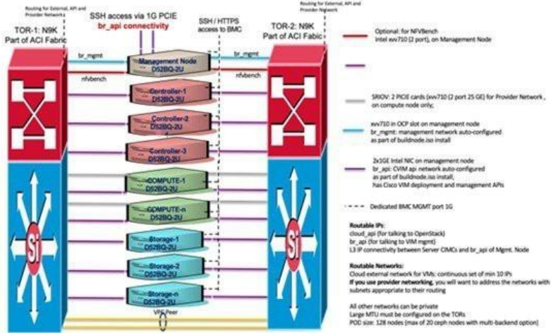
Quanta (D52BQ-2U) Fullon Pod with 25GE Intel NIC (xxv710)
